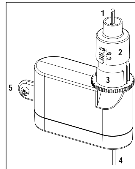
Figure 3: Rain/Freeze Transmitter
