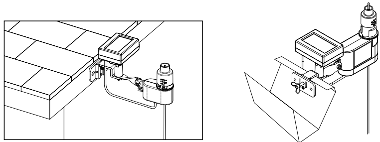
Figure 8: Attaching Sensor/Transmitter to gutter or flat surface
