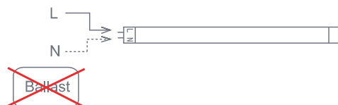
Diagram 3 – Single tube wiring
