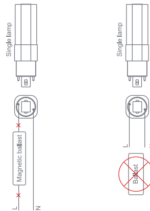
Diagram 3 – Magnetic ballast fixture wiring modification
